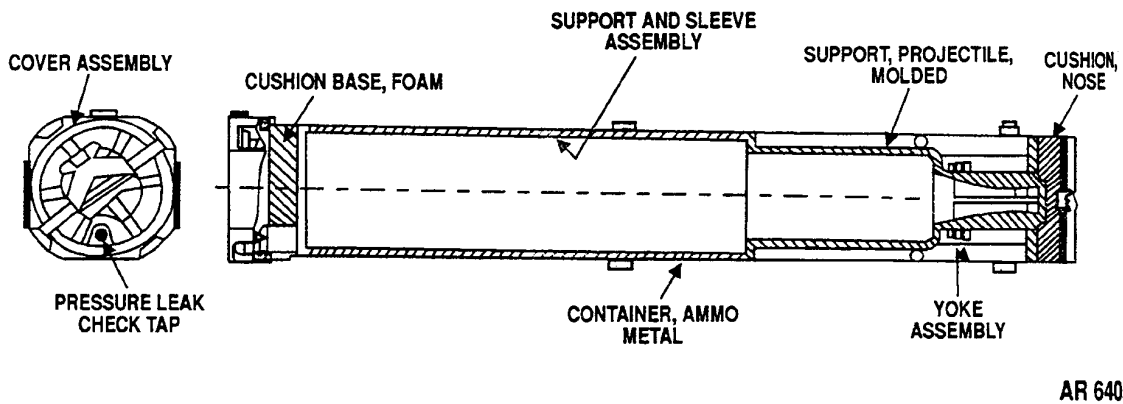
Figure 3-29. Metal Container for Cartridge, 120mm: HEAT-MP-T, M830A1 and HE-OR-T, XM908.
